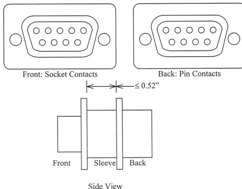
Figure 1. Adapter Configuration
